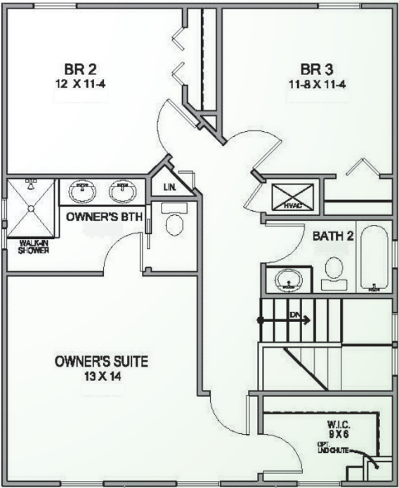
SECOND FLOOR
